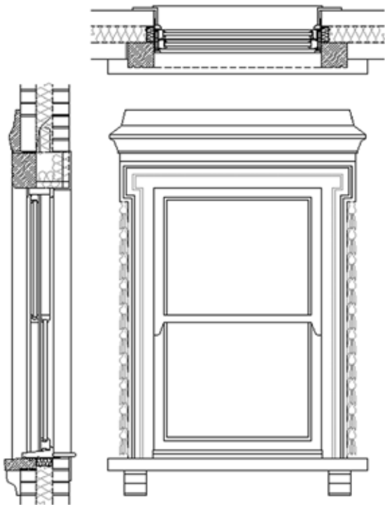
Above: A window detail in plan, section and elevation for a residential refurbishment scheme in London
